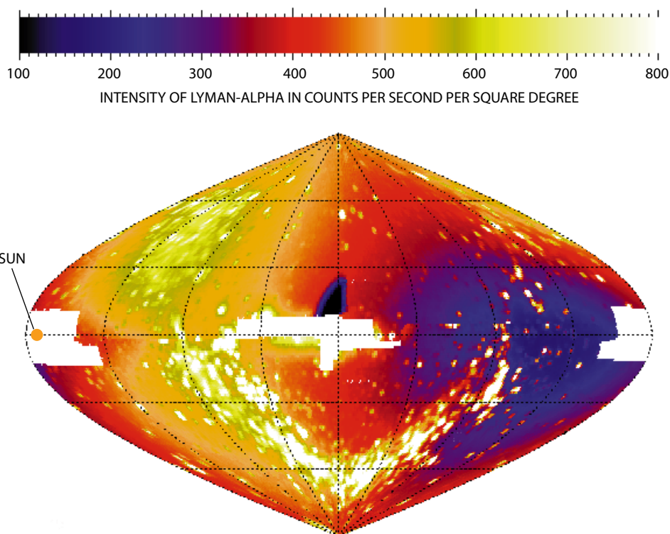
INTERSTELLAR HYDROGEN glows in the ultraviolet light of the Lyman-alpha spectral line at a wavelength of 1,216 angstroms. An interstellar cloud of gas emits the diffuse regions, and hot stars produce the bright dots. The sun travels through the cloud at a velocity of 26 kilometers per second, and the solar wind creates an asymmetry in the diffuse UV glow.
